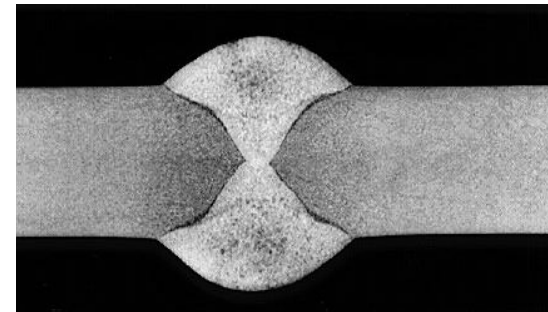
75% Argon / 25% Helium
