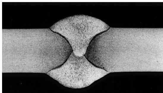
50% Argon / 50% Helium
