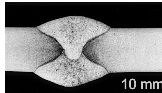
25% Argon / 75% Helium
